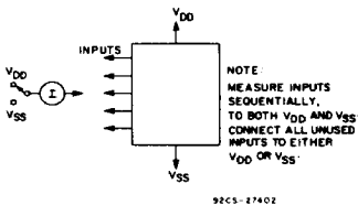
Fig.11 — Input leakage test circuit.
