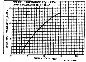
Fig.8 — Typical maximum clock input frequency vs. V_{DD} .
