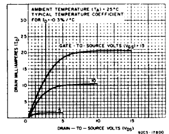
Fig.2 — Typical n-channel drain characteristics.
